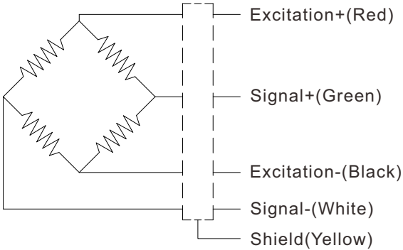
Wiring Code@Compression
